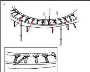
Strap with "S" hook on the pad edge Cross the strap over the top rail frame to hook the V ring
