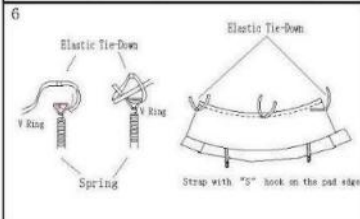
Strap with "S" hook on the pad edge Cross the strap over the top rail frame to hook the V ring
